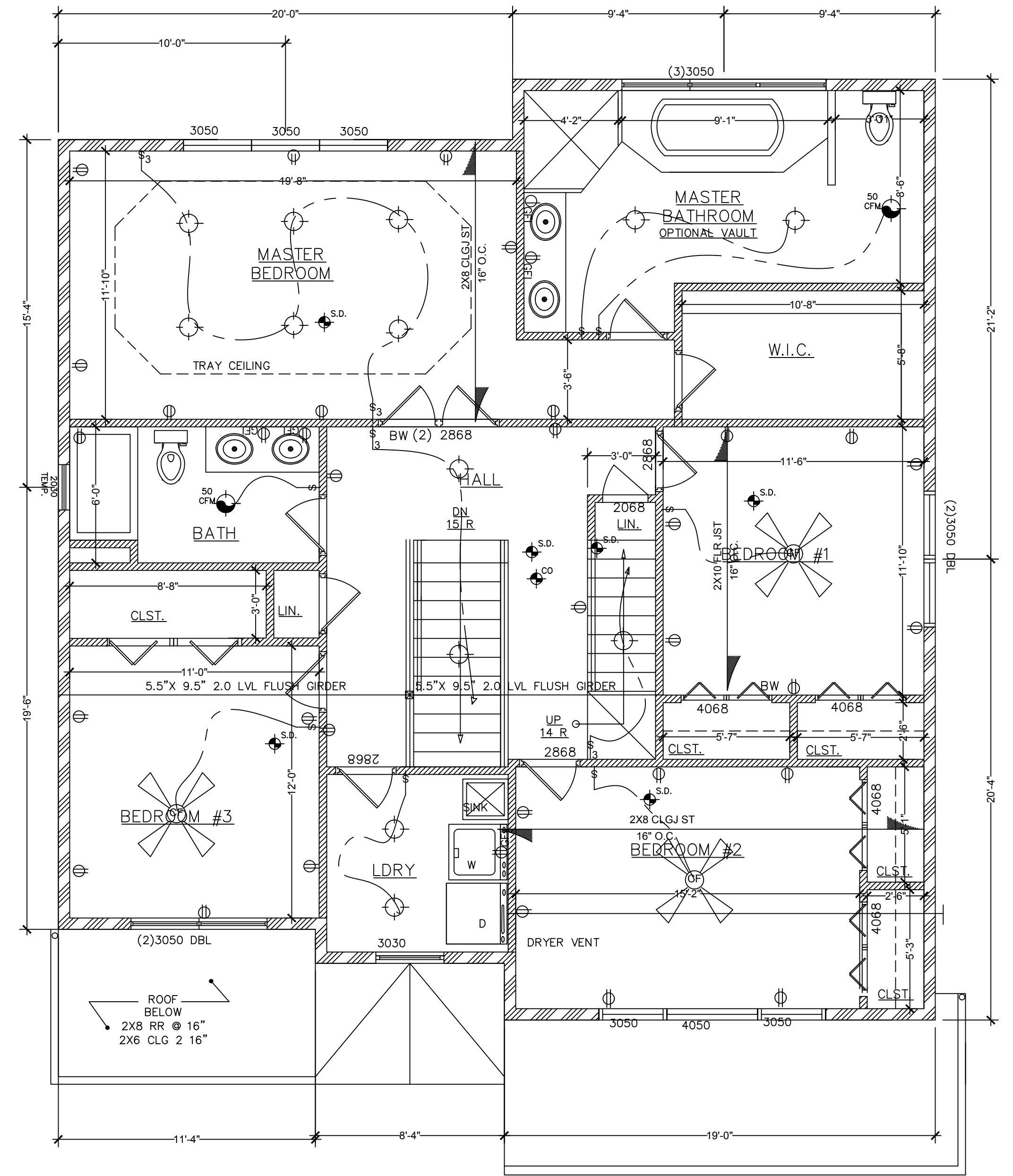
SECOND FLOOR PLAN Scale: 1/4" = 1'-0"
