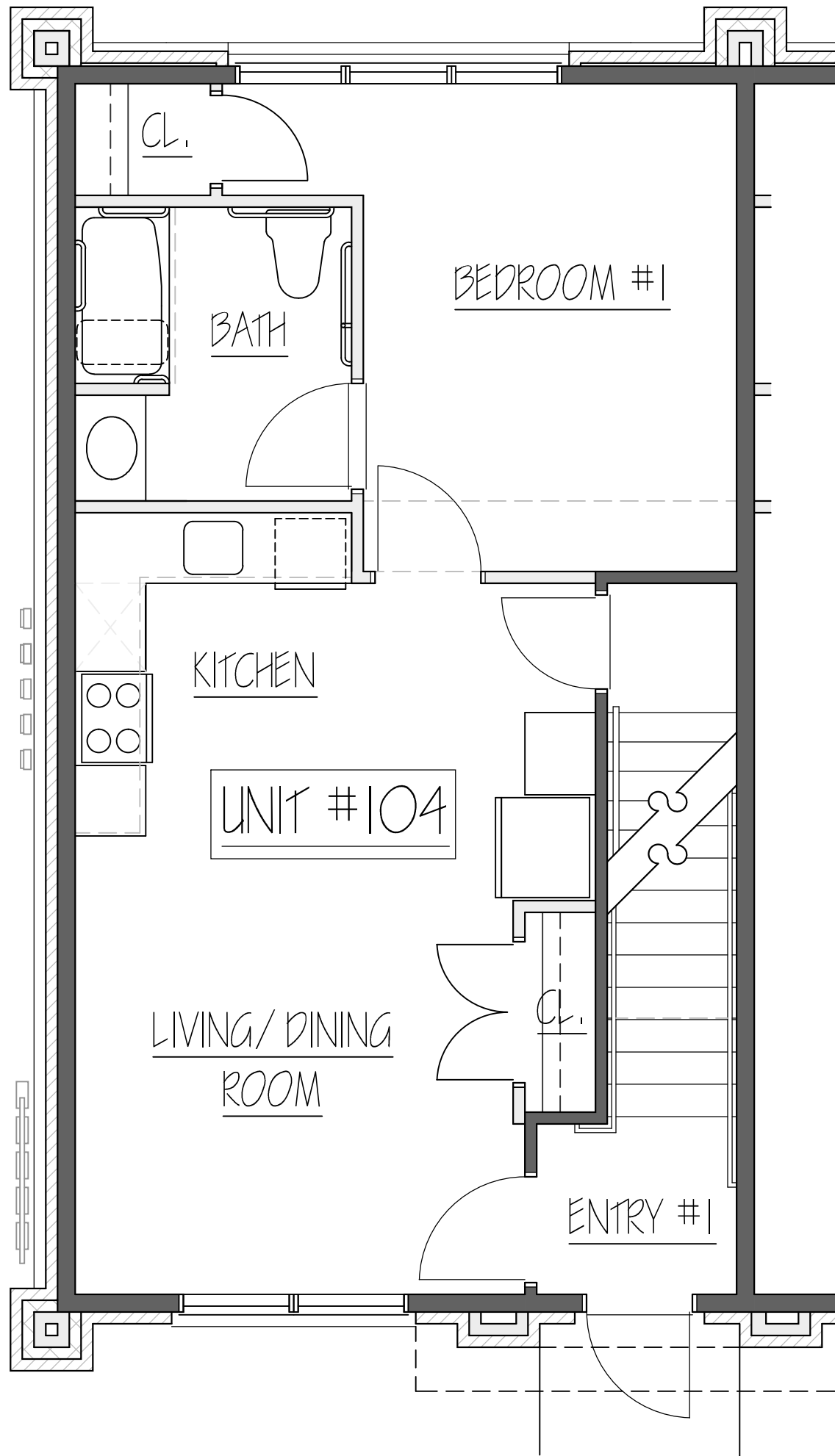
MAIN FLOOR PLAN (UNIT 104-106)
